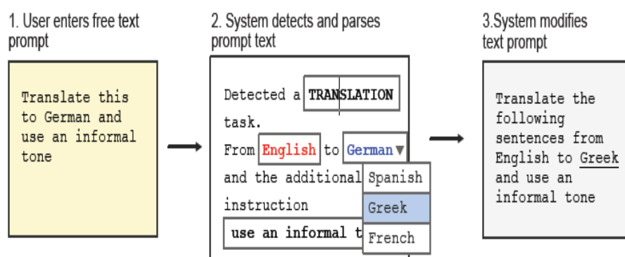
Fig. 12. GUI example.
