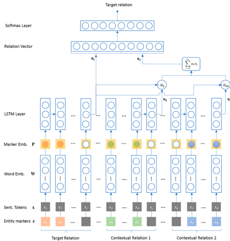
Fig. 34. The architecture of the context aware RE
